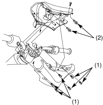
HANDLEBAR
