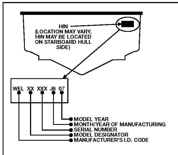
Hull Identification Number Location
