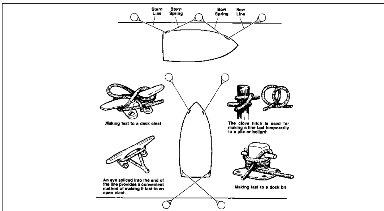
FIGURE 7.4 MOORING LINES
