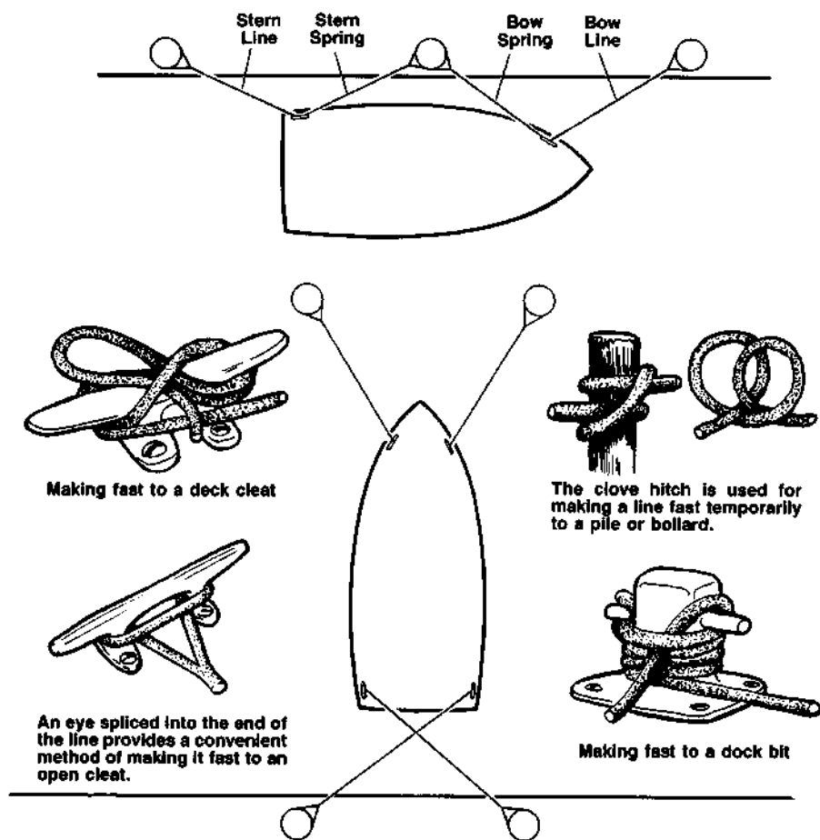
FIGURE 10.5 MOORING LINES
