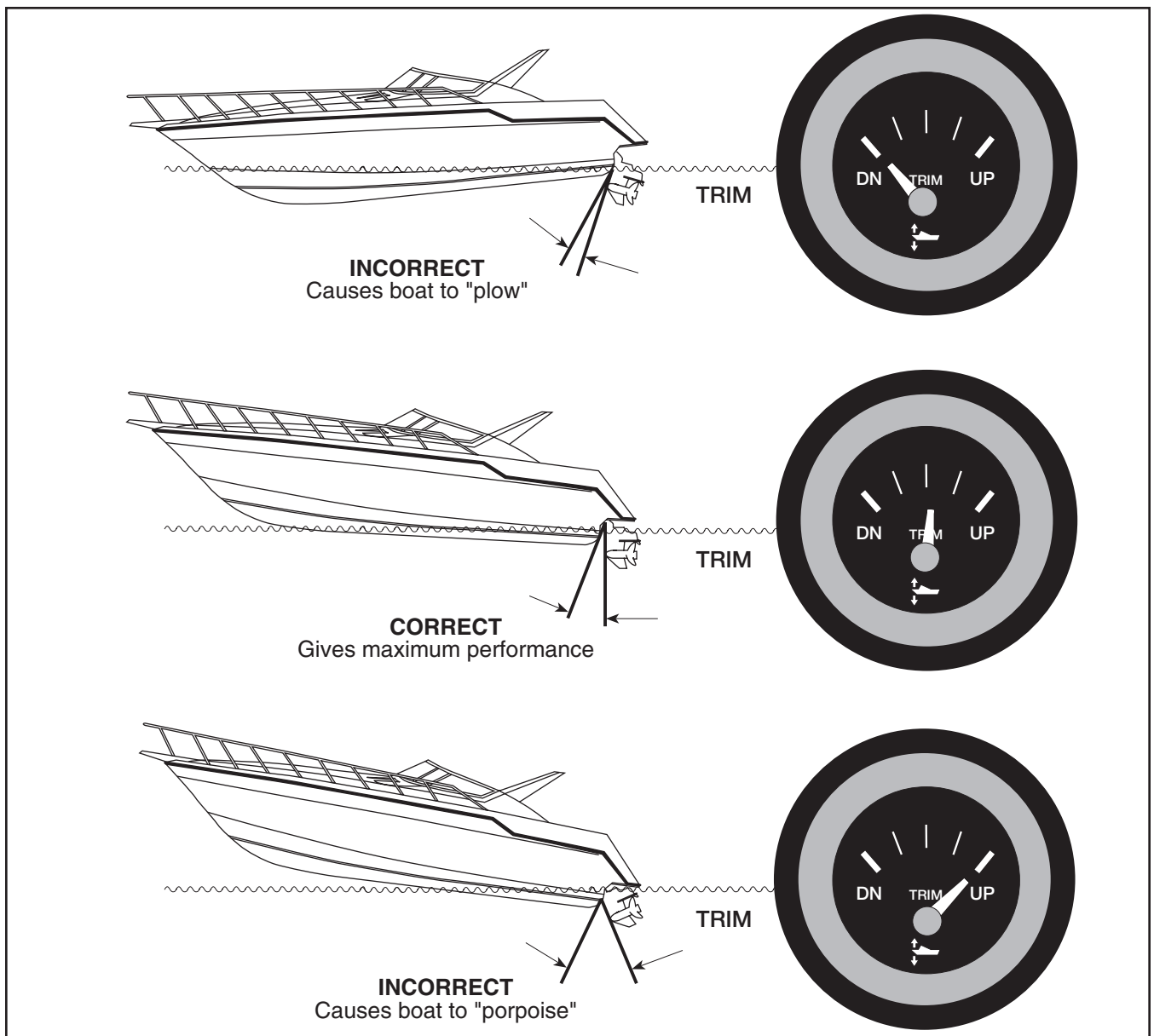
FIGURE 10.3 TRIMMING THE BOAT OUTDRIVE
