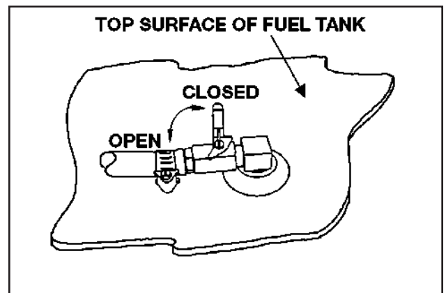
FIGURE 5.1 FUEL SHUTOFF VALVE (SINGLE ENGINE BOATS ONLY)
