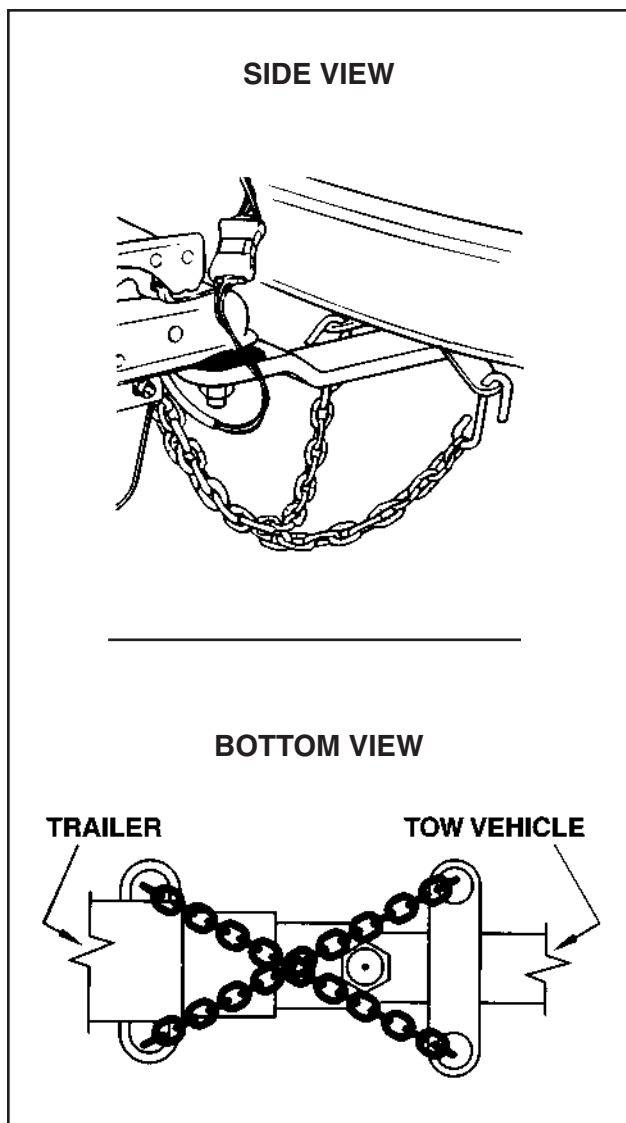
FIGURE 13.1 SAFETY CHAINS
