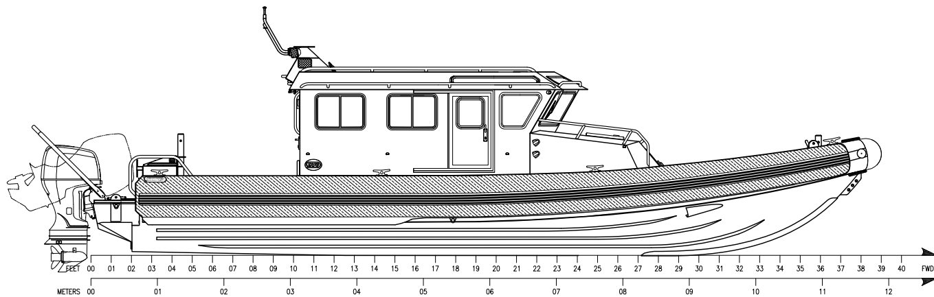
OUTBOARD PROFILE
