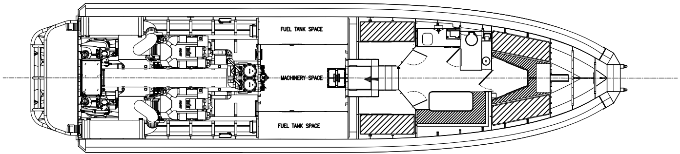
INBOARD PLAN VIEW
