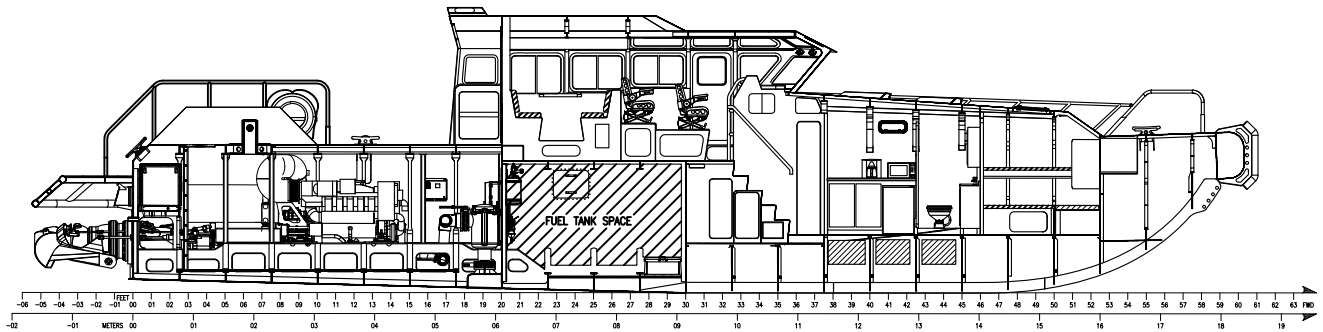
INBOARD PROFILE
