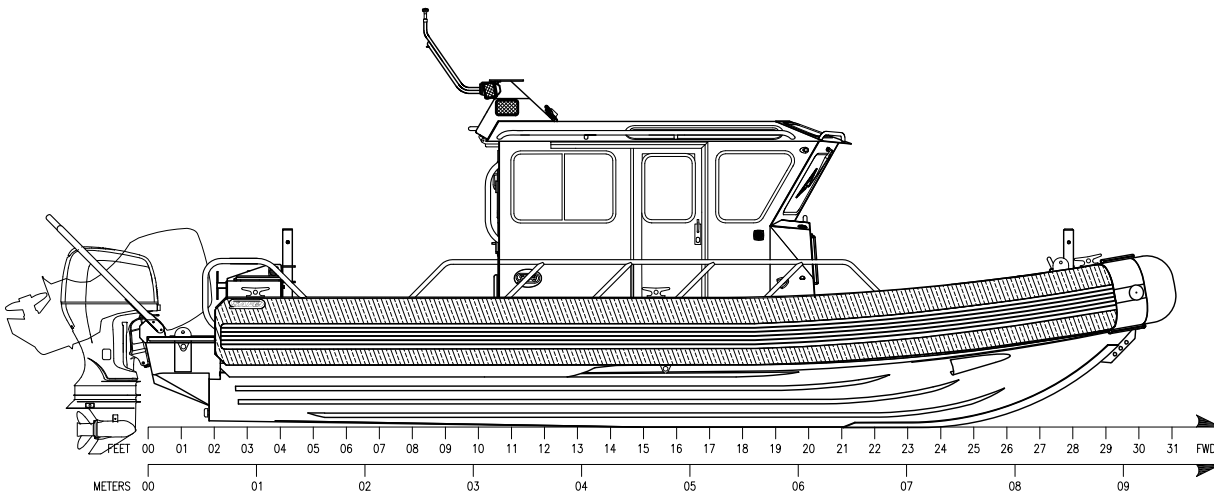
OUTBOARD PROFILE
