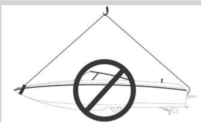
INCORRECT HOISTING
