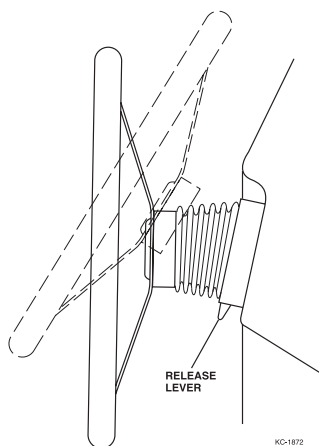
Figure 2-31. Tilt Steering
