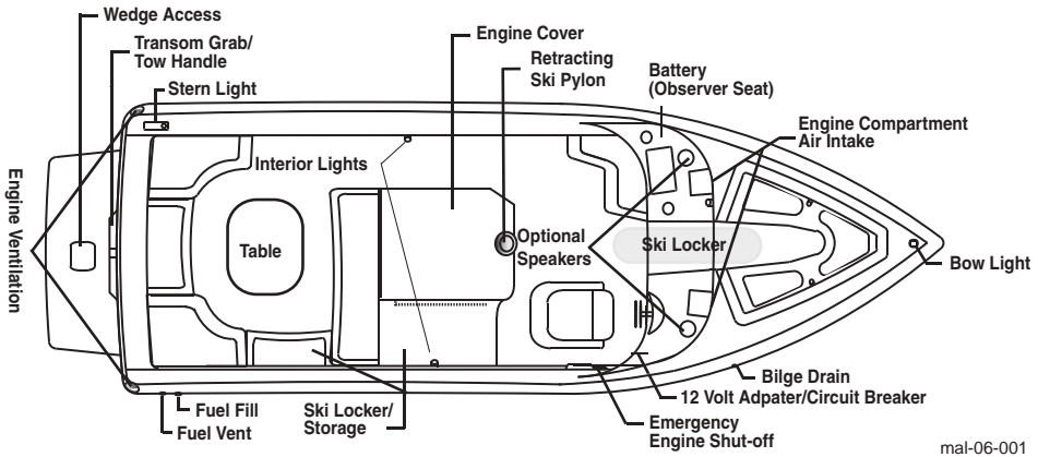
Figure 2-1. General Layout XTi Model Boats
