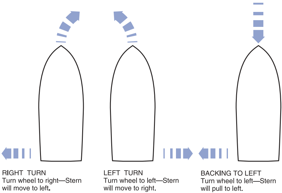
Figure 3-8. Turning With A Rudder
