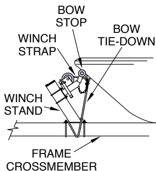
Figure 32 - Bow Tie-Down
