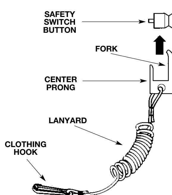
FIGURE 2.8 TYPICAL IGNITION INTERRUPTER WITH LANYARD
