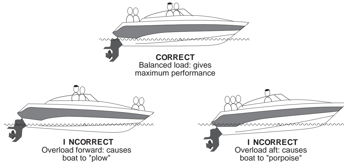
FIGURE 3.2 – LOADING PASSENGERS
