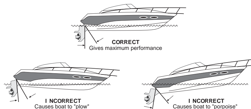
FIGURE 3.3 – TRIM / MOTOR ANGLE
