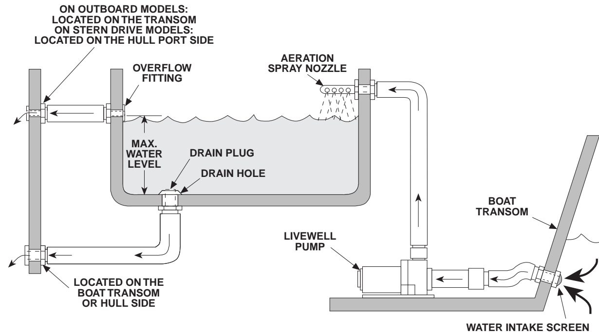
FIGURE 2.9 MANUAL LIVEWELL
