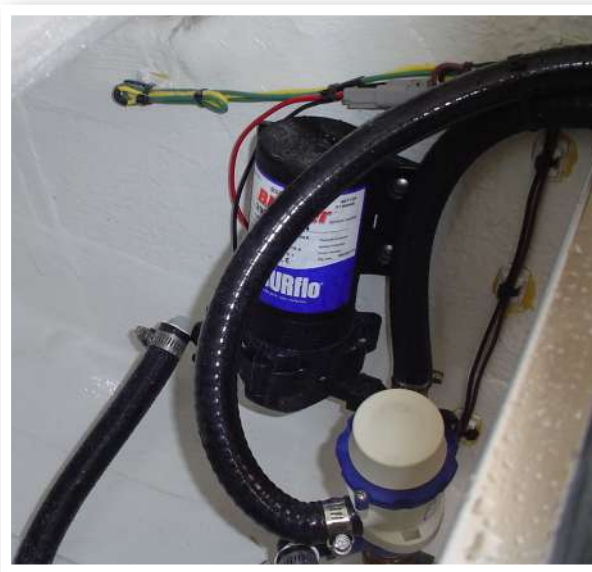
Raw Water Pump
