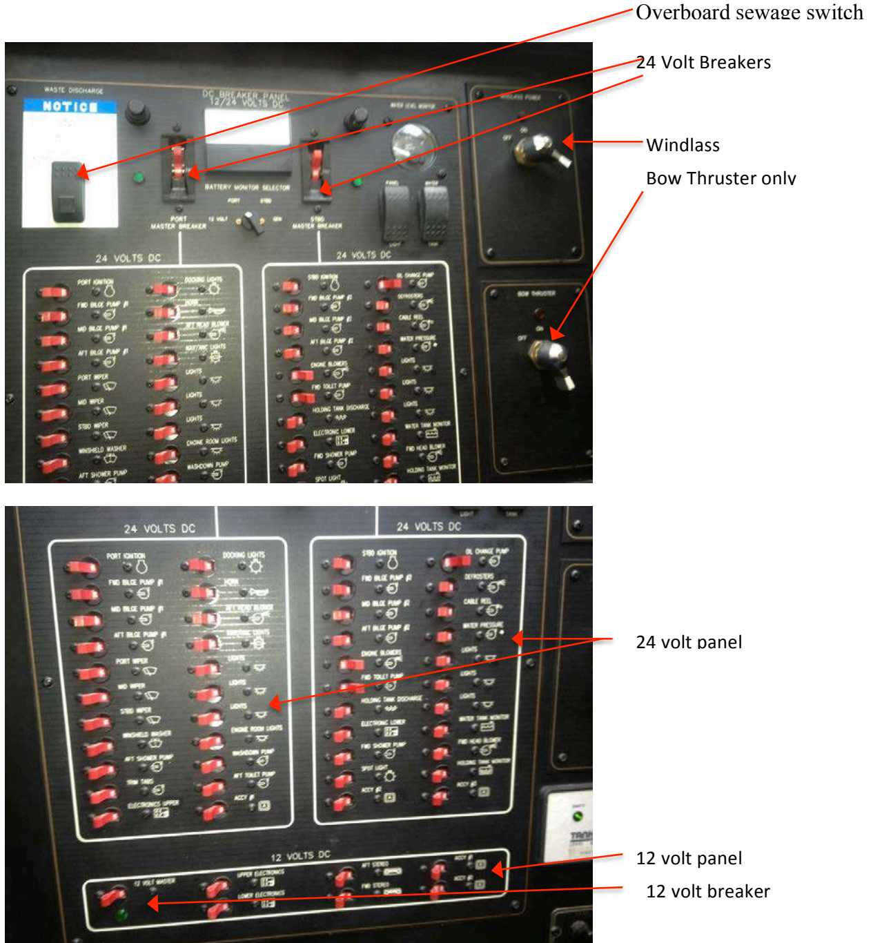
24 Volt Battery power panel
