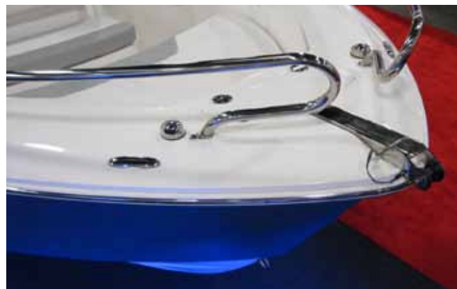
Anchor/Rope Locker and Roller Assembly
